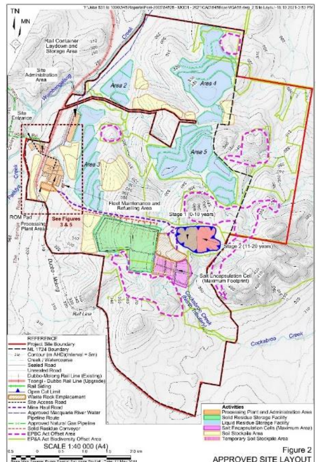
Approved Dubbo Project site layout.
